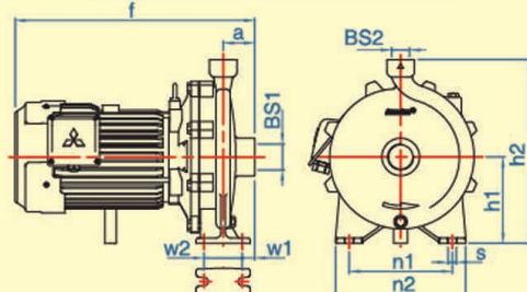
WCH-3705S / WCH-3705T
